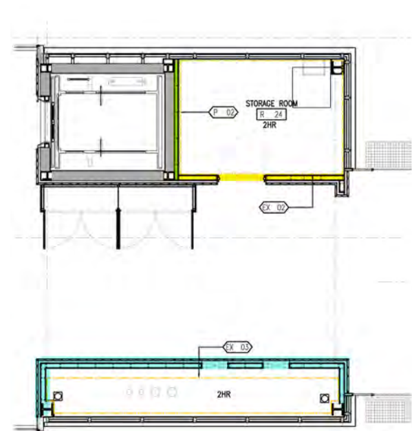
005 ENTRANCE PODS FOOTBRIDGE LEVEL (Type b) DRYWALL & FIRE COMPARTMENTATION KEY PLAN LAYOUT 1:50
