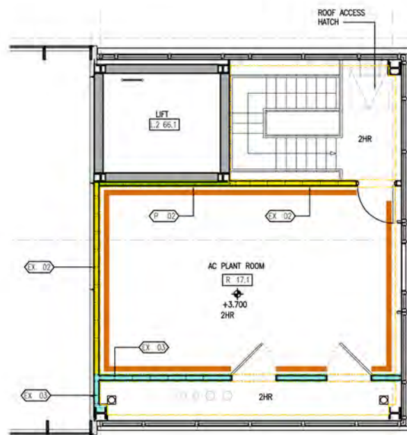
002 ENTRANCE PODS AC PLANT ROOM LEVEL (Type a & b) DRYWALL & FIRE COMPARTMENTATION KEY PLAN LAYOUT 1:50
