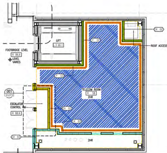
003 ENTRANCE PODS FOOTBRIDGE LEVEL (TELECOM ROOM) DRYWALL & FIRE COMPARTMENTATION KEY PLAN LAYOUT 1:50
