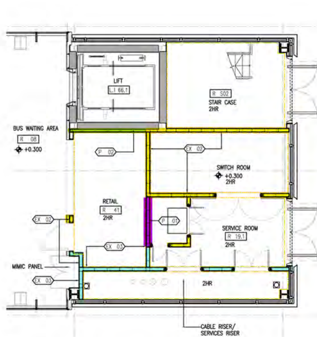
001 ENTRANCE PODS GROUND LEVEL (Type a & b) DRYWALL & FIRE COMPARTMENTATION KEY PLAN LAYOUT 1:50
