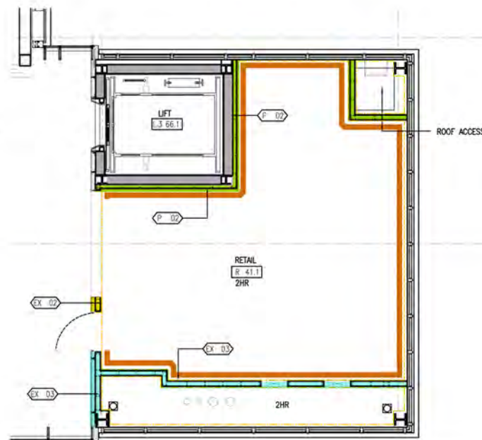
004 ENTRANCE PODS AC PLANT ROOM LEVEL (RETAIL) DRYWALL & FIRE COMPARTMENTATION KEY PLAN LAYOUT 1:50
